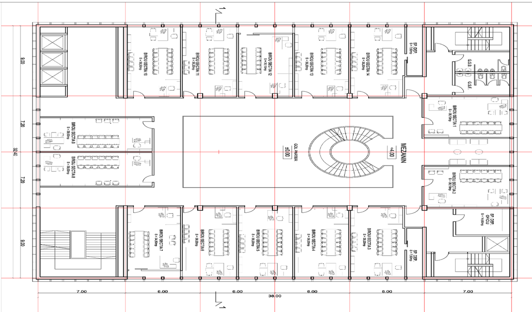
PLAN MAZANIN SC:1/100 Suprafata mezanin = 1.140mp
